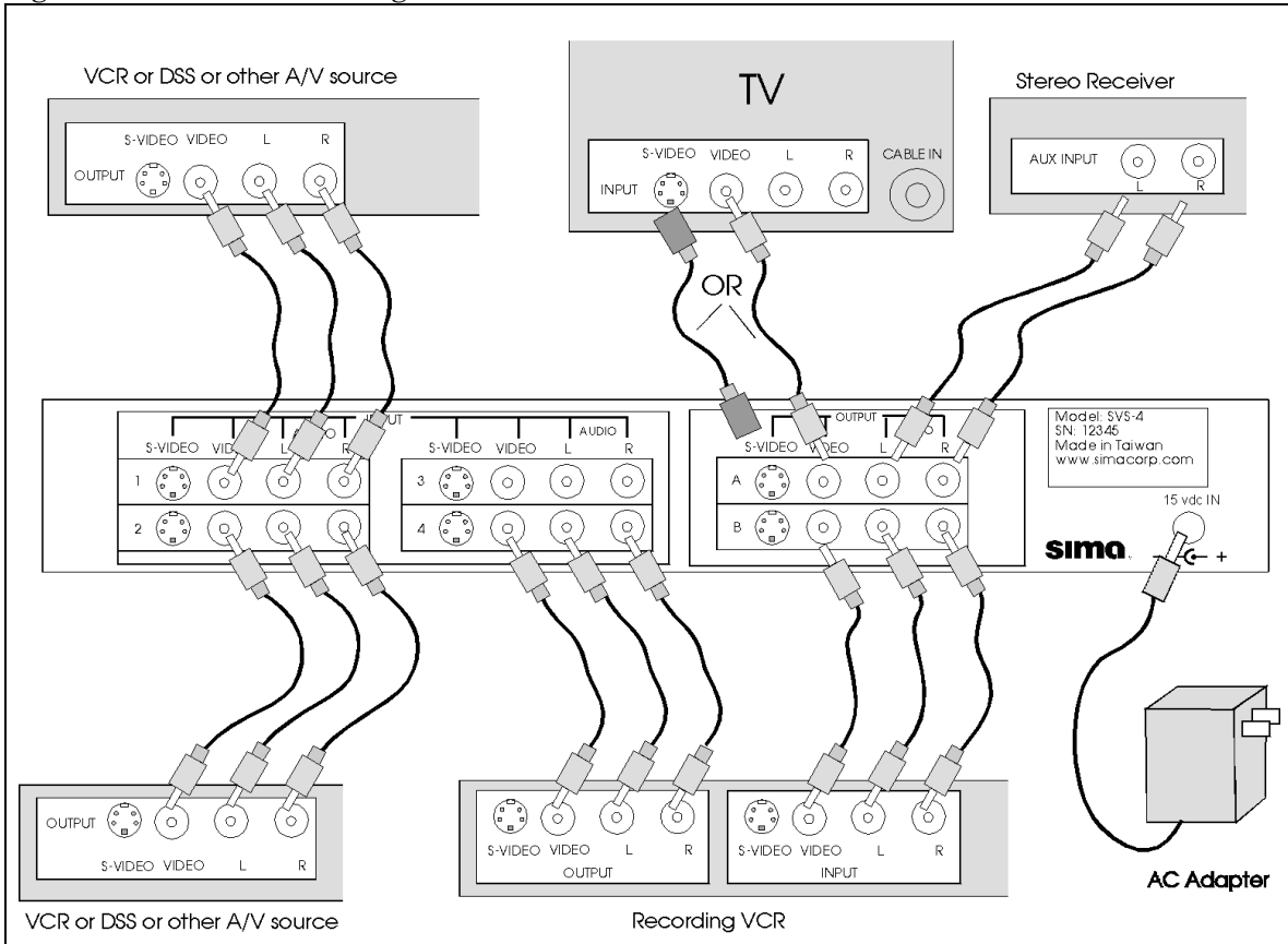
Figure 6, SVS-4 with recording VCR
