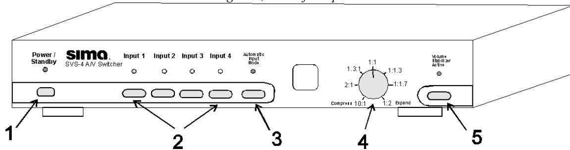
Figure 1, SVS-4 front panel
