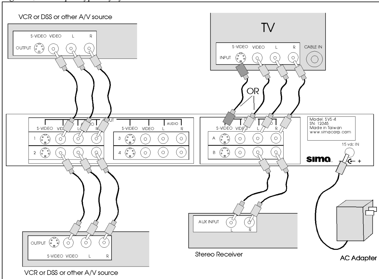
Figure 5, Hook-up in typically system
