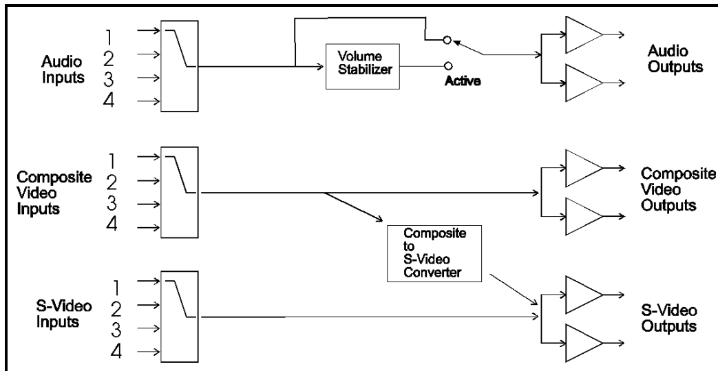
Simplified Block Diagram of the SVS-4
