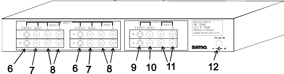
Figure 2, SVS-4 rear panel
